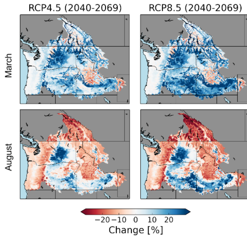
Figure 14. March (top) and August (bottom) average soil moisture percent change relative to historical period (1970-99) for 10-model ensemble average.
