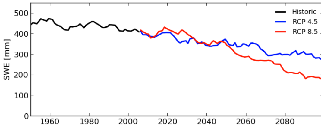
Figure 11. 10-model ensemble average SWE monthly time series averaged over the PNW (5-year moving average).
