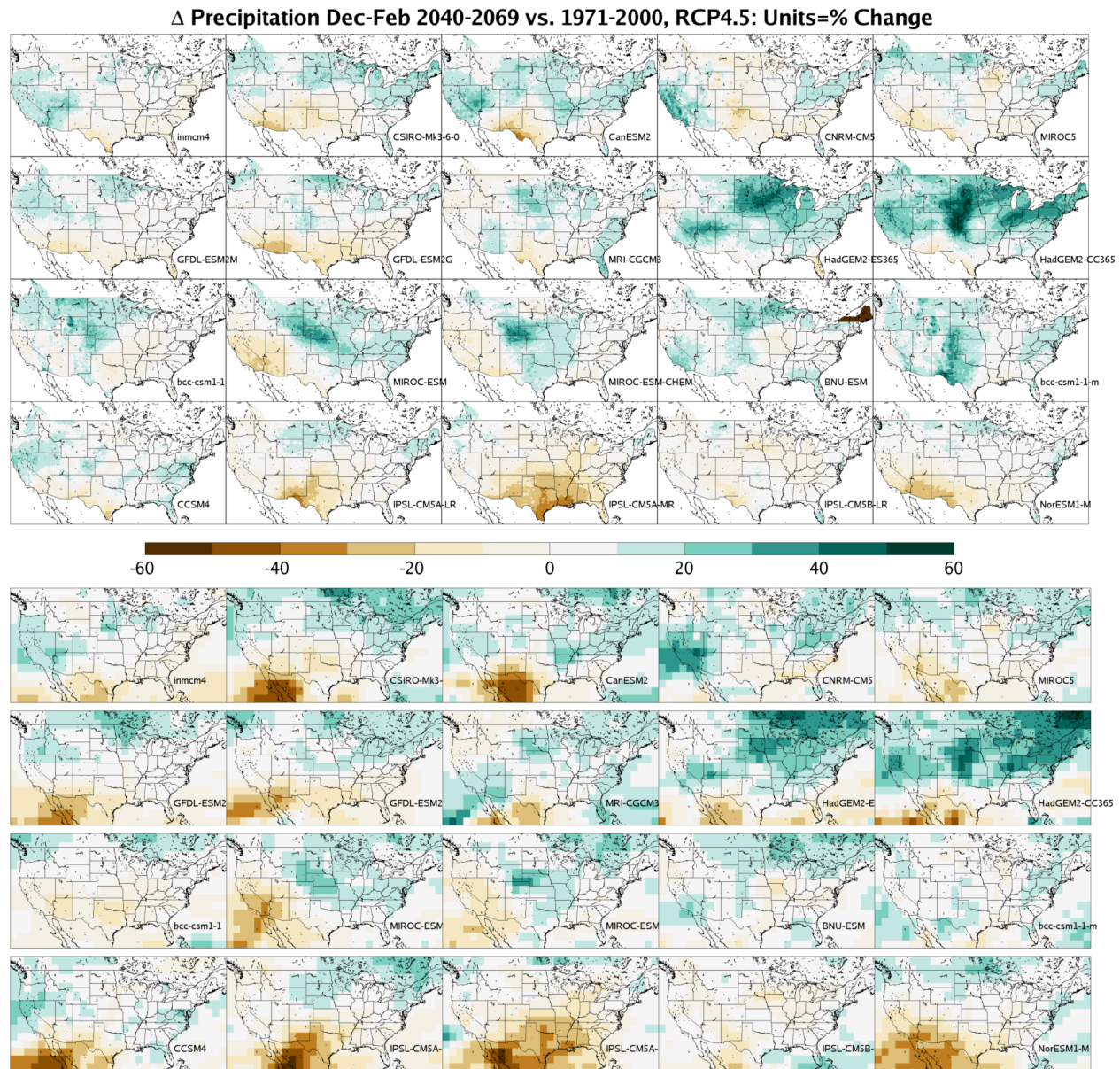
Figure 3. Projected changes in mean Dec-Feb precipitation from the years 1971-2000 to the years 2040-2069 of experiment RCP4.5 for the (top) downscaled and (bottom) raw 20 CMIP5 climate models.
