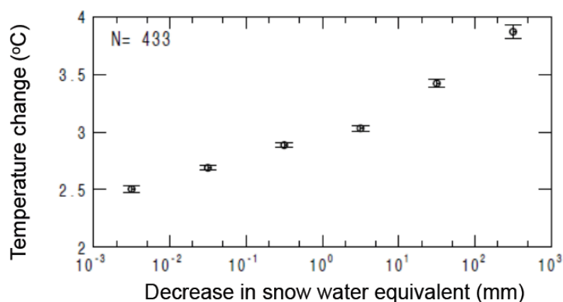
Figure 6. Mean spring temperature change, against the decrease in April snow water equivalent (SWE) (2030-2049 minus 1986-2005). Values from all grid points in the Pacific Northwest were binned by change in the mean April SWE. Error bars show +/- 1 standard deviation.
